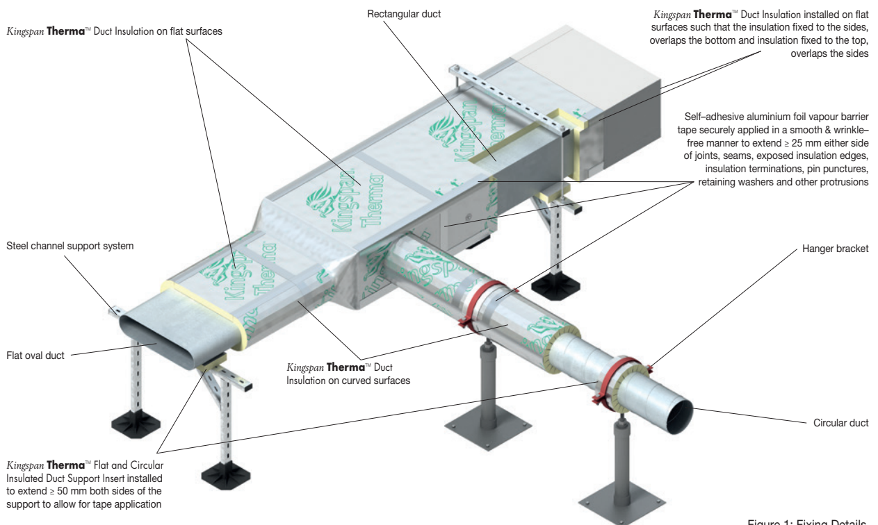
Figure 1: Fixing Details
